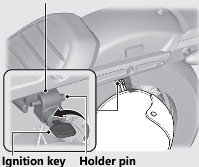
Helmet holder
